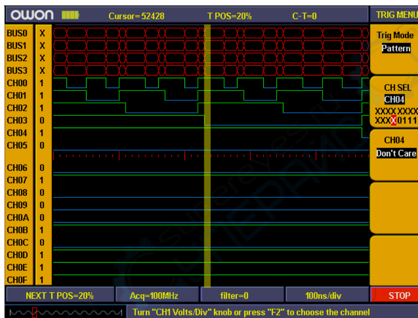
Fig.5-59: Pattern trigger
