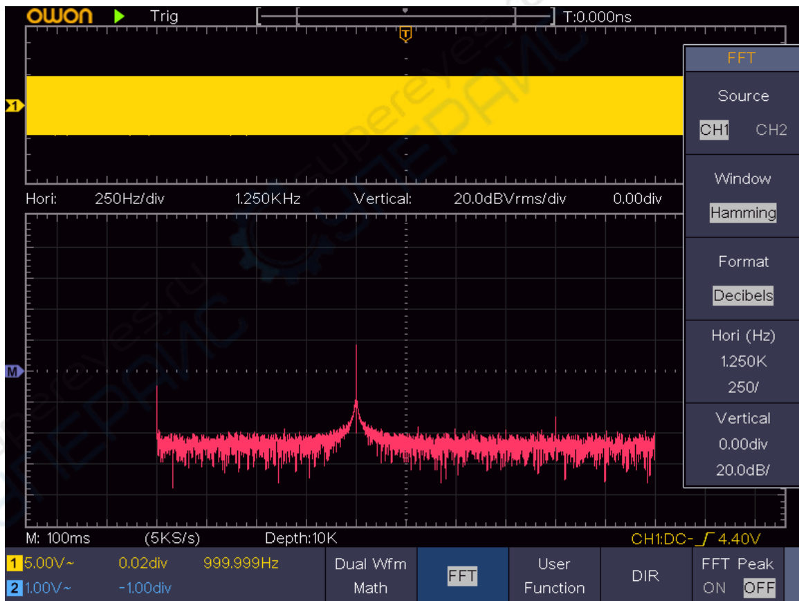
Figure 4-1 Hamming window
