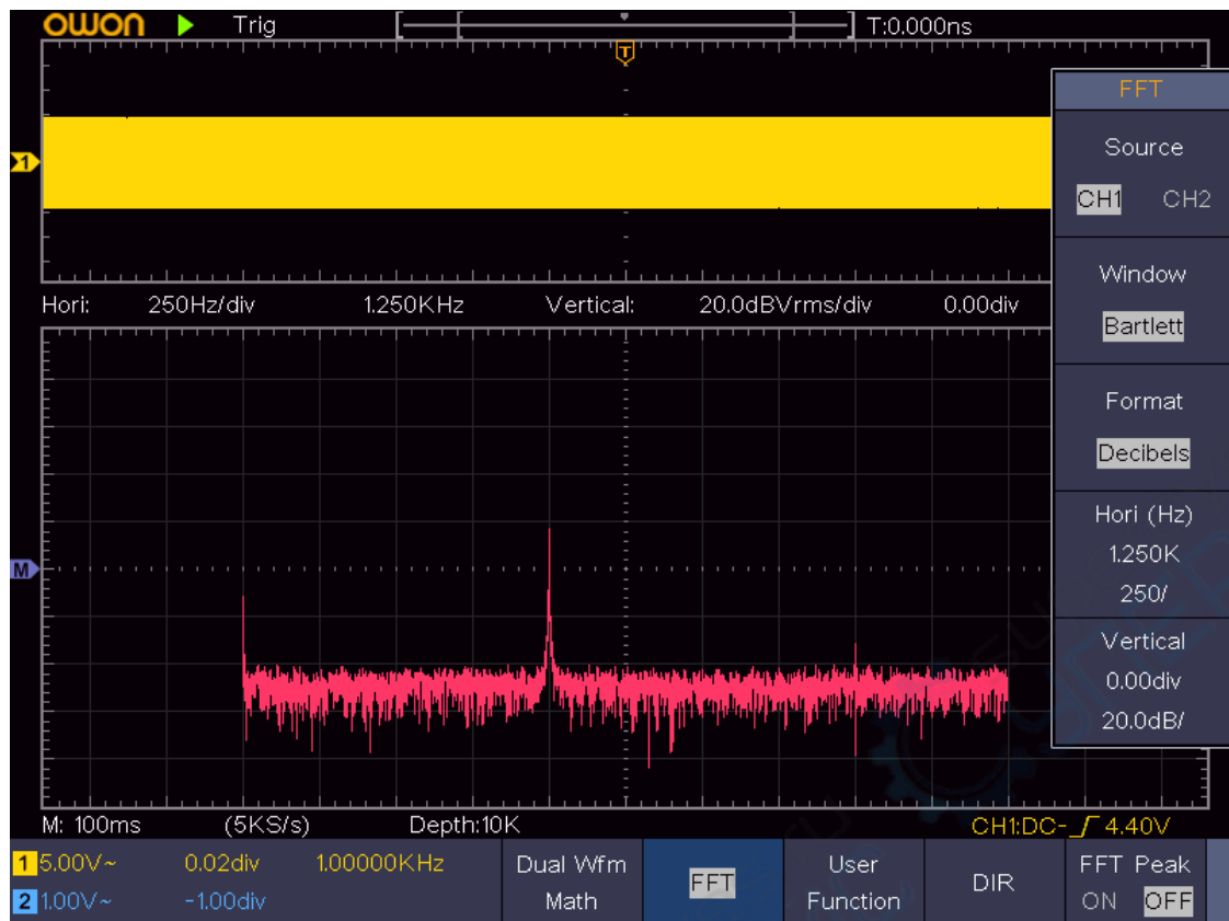
Figure 4-6 Bartlett window
