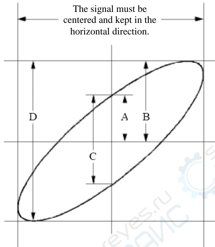
Figure 9-6 Lissajous Graph
